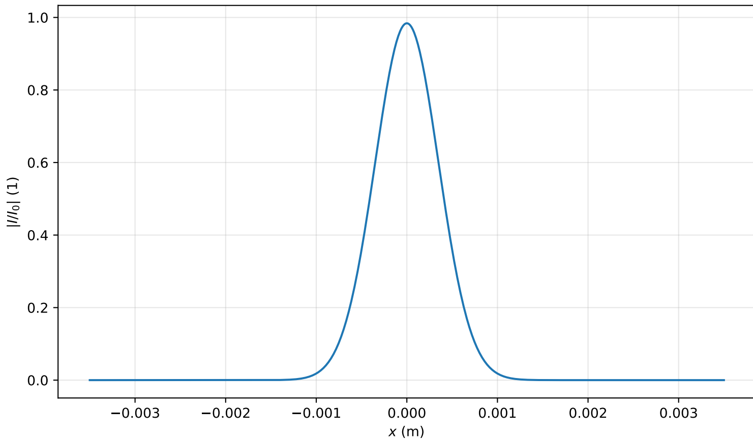
Intensity profile I(x, y = 0, z = 0.318m)/I_0 , P_{in}=0.1P_{cr} , artificial time
